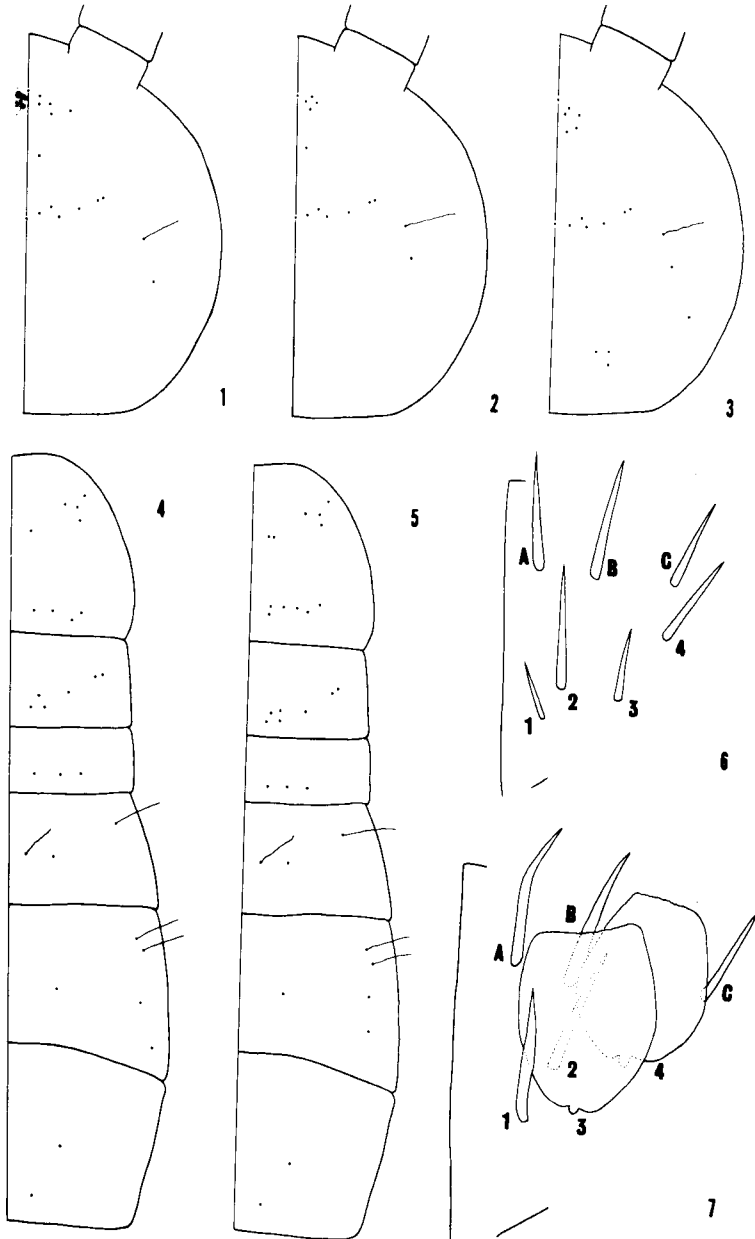
Figs. 1-7, Heteromurus sp. Fig. 1. H. (Alloscopus) tetraacanthus -Dorsal head macrochaetotaxy and distribution of lasiotrichia, each dot represents one seta. Fig. 2. H. (A.) tenuicornis -Dorsal head macrochaetotaxy and distribution of lasiotrichia. Fig. 3. H. (Heteromurus) schoetti Denis-Dorsal head macrochaetotaxy and distribution of lasiotrichia based on specimens from Guatemala. Fig. 4. H. (A.) tetraacanthus -Dorsal body macrochaetotaxy. Fig. 5. H. (A.) tenuicornis -Dorsal body macrochaetotaxy. Fig. 6. H. (A.) tetraacanthus -Chaetotaxy of base of labium. Fig. 7. H. (A.) tenuicornis -Chaetotaxy of base of labium.
