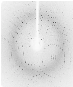
X-ray diffraction pattern from Lucina pectinata hemoglobin.
