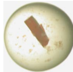
Hemoglobin crystal from Lucina pectinata .
