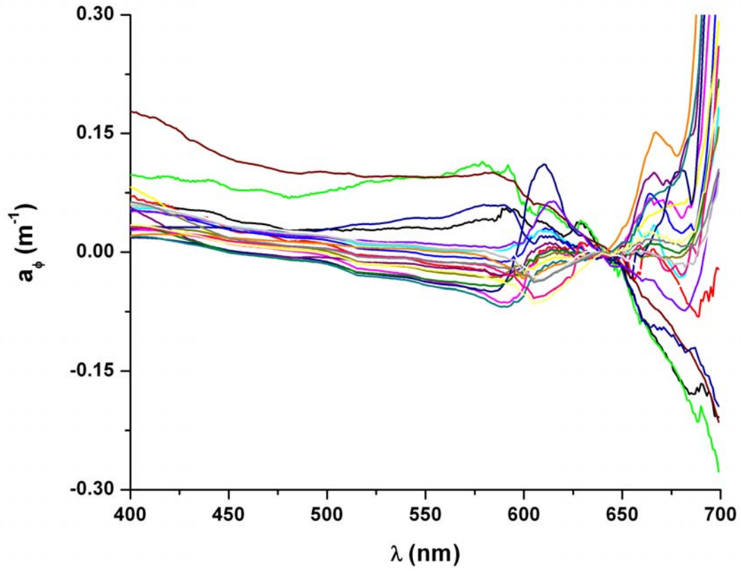
Figure 48. Spectral phytoplankton absorption coefficients [ a_{\phi}(\lambda) ] obtained from the QAA for the TSS < 5 \text{ mg/l} data set in Mayagüez Bay.
