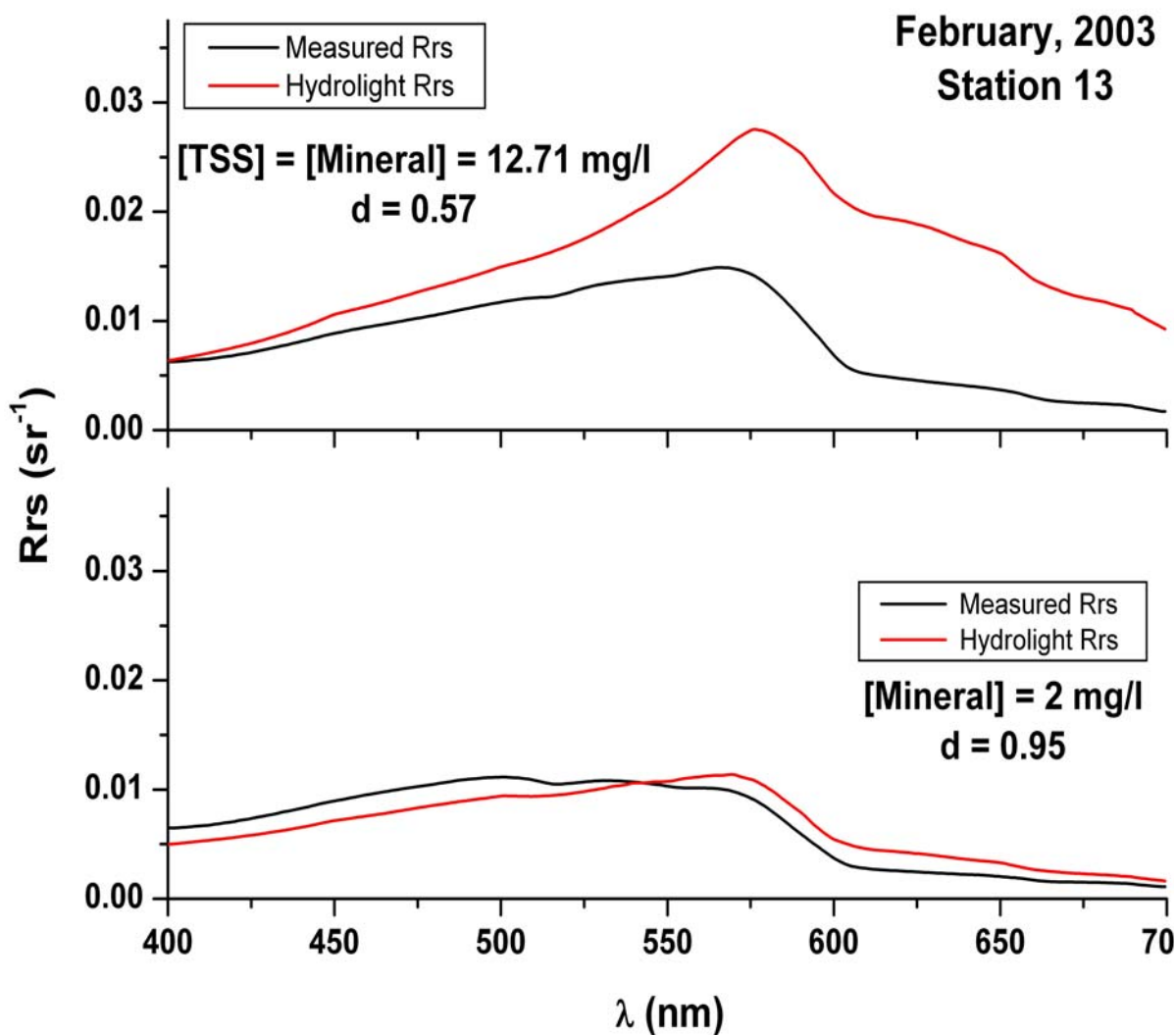
Figure 23. Model fit when TSS was used to estimate mineral concentration (upper graph) and when mineral concentration was iteratively adjusted to 2 \text{ mg l}^{-1} . The increase in Willmott's Index of Agreement suggests that the mineral fraction of the TSS was small (about 16%) for this particular sample.
