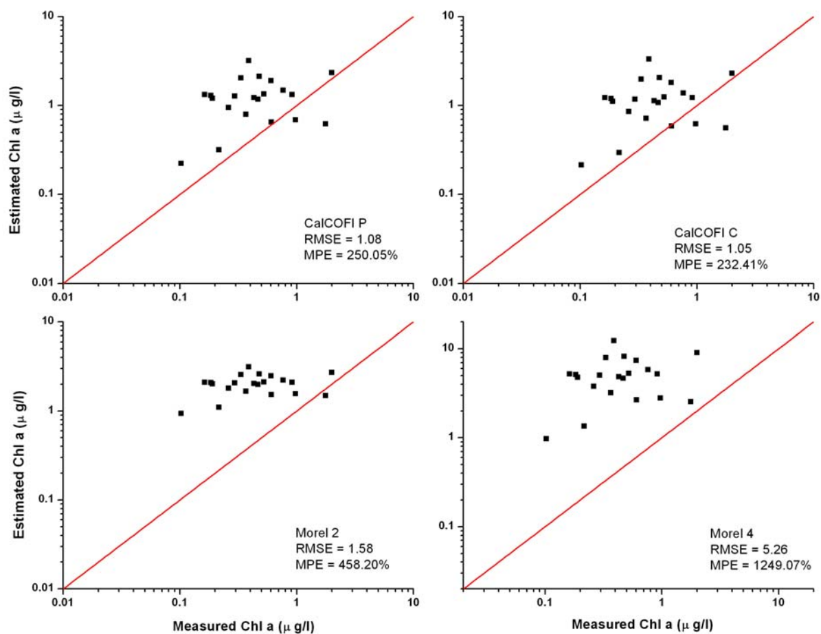
Figure 32. Chl a estimated by CalCOFI P, CalCOFI C, Morel 2 and Morel 4 empirical algorithms versus measured Chl a for the data subset TSS < 5 mg/l (RMSE in \mu g l -1 ).
