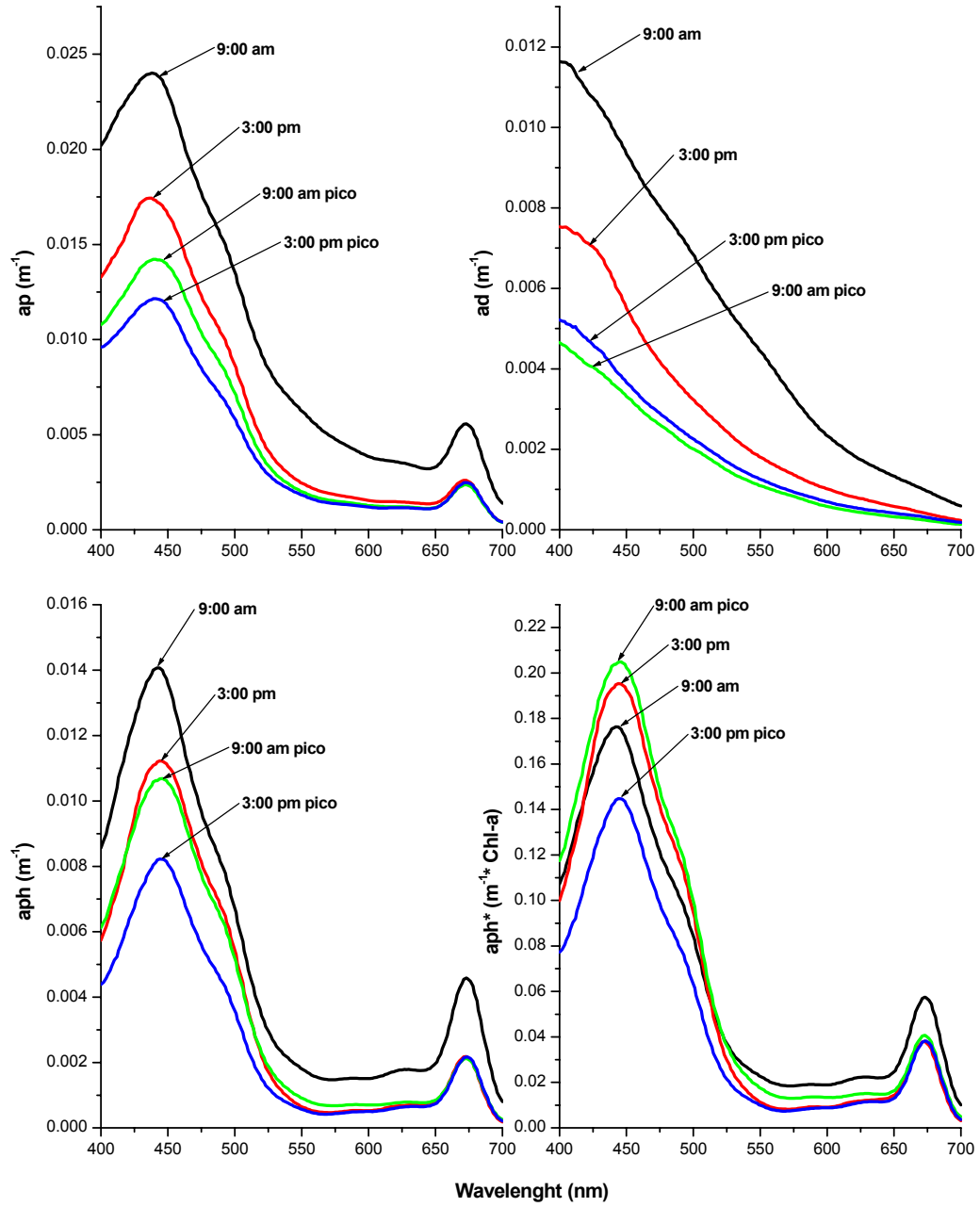
Figure 49. Absorption spectra of a_p , a_d , a_{ph} , and a_{ph^*} for the surface stations of Mona for total phytoplankton and picoplankton.
