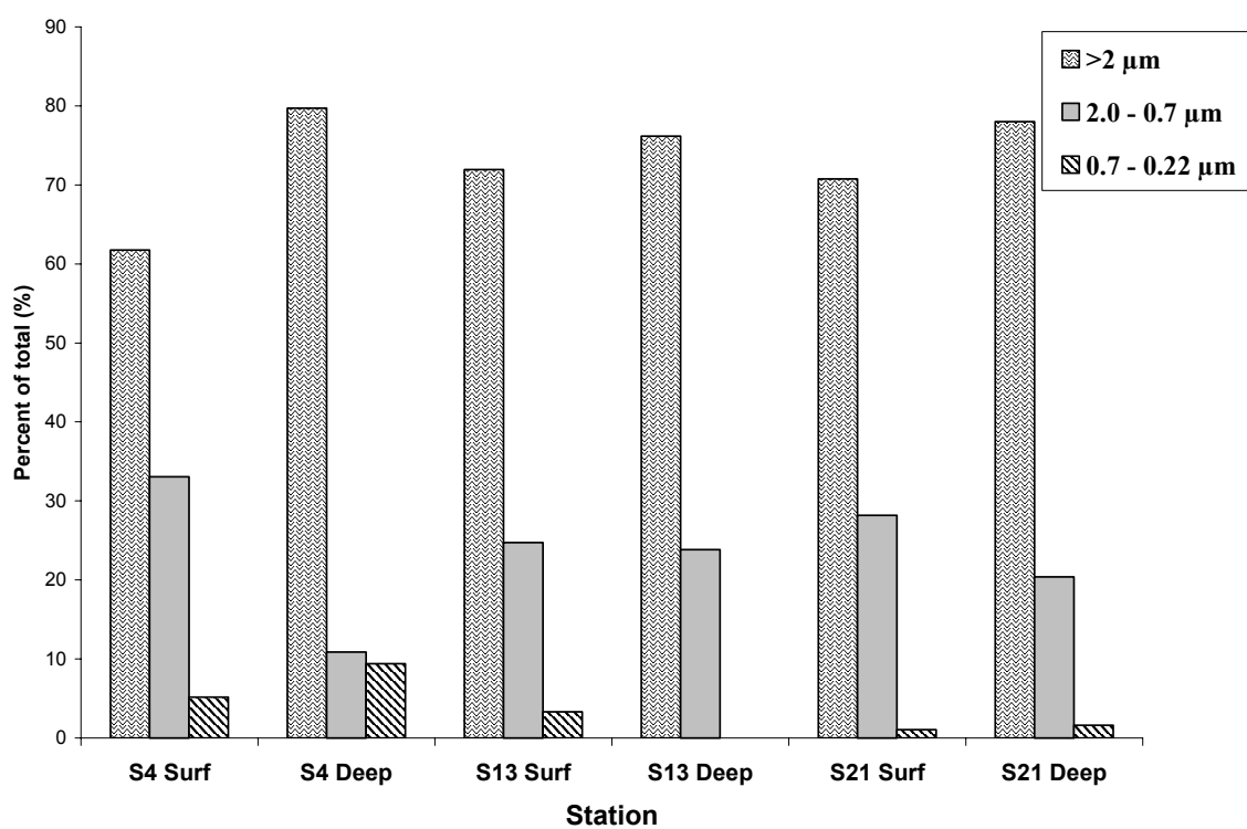
Figure 23. Percent of phytoplankton belonging to the different size classes at the Mayagüez Bay stations during the October 2001 cruise.
