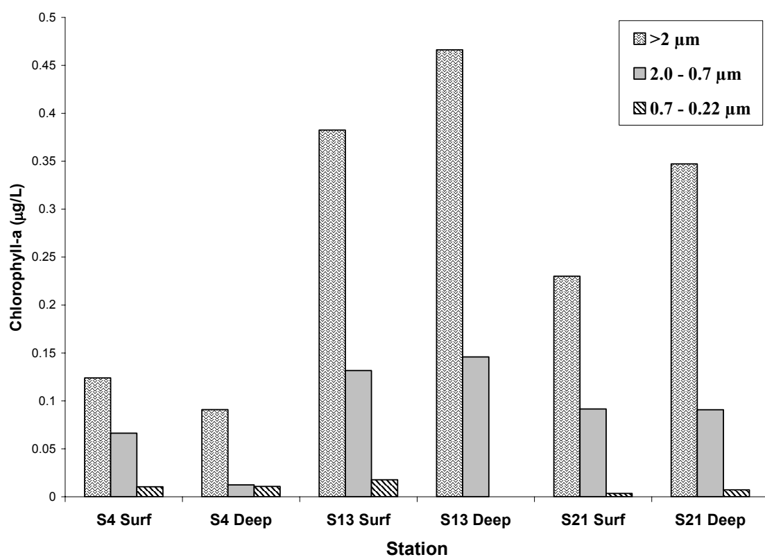
Figure 24. Chlorophyll-a concentration accounted for by the different size classes of phytoplankton at the Mayagüez Bay stations during the October 2001 cruise
