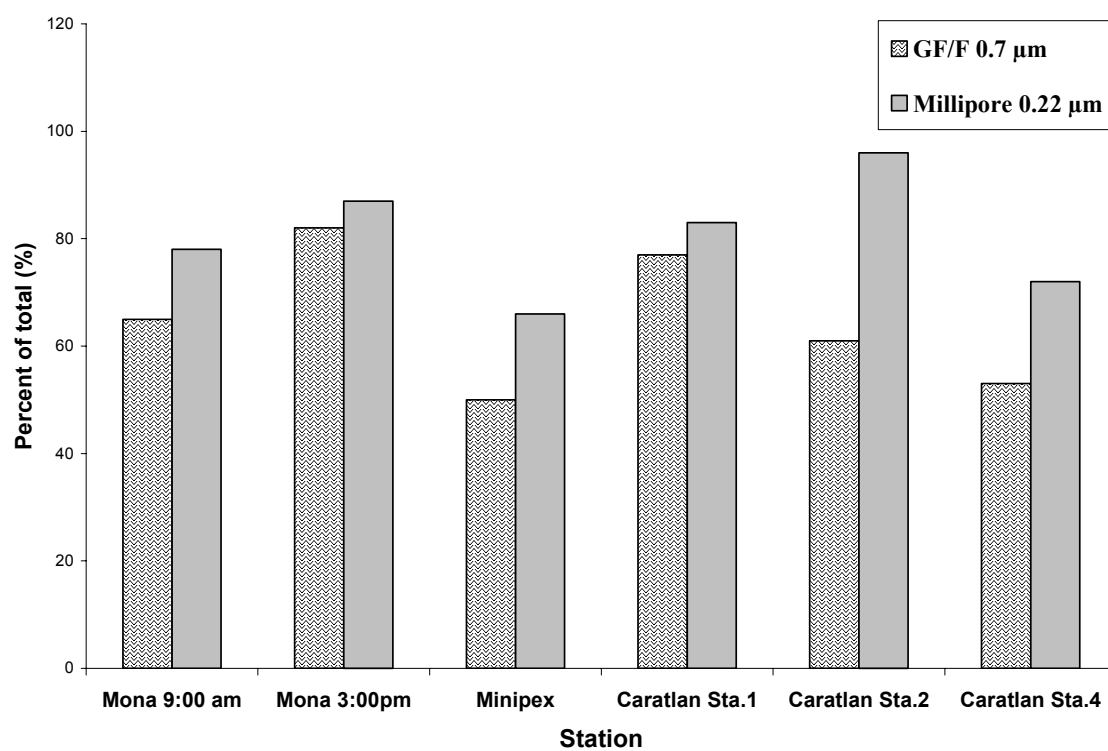
Figure 11. Percent of the total phytoplankton population retained by the different filters, after pre-filtration with a 2.0 µm filter, in oceanic surface samples.
