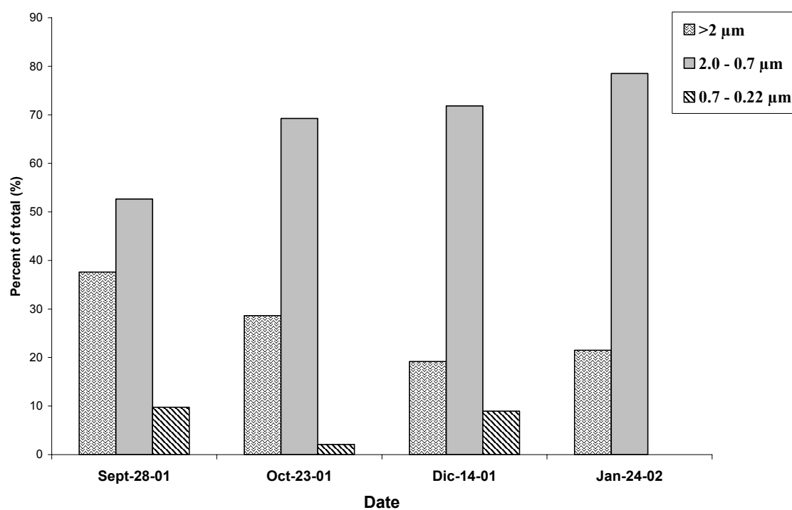
Figure 17. Percent of phytoplankton belonging to the different size classes at CaTS DCM.
