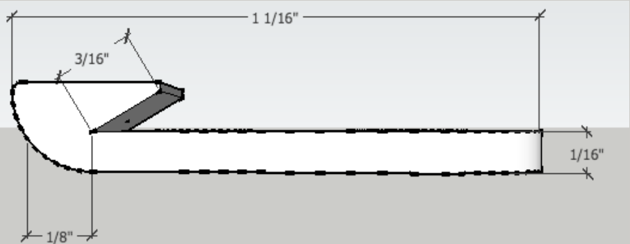
Left View
